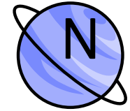
Neptune
